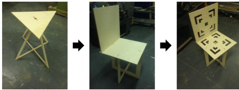
Figure 2 Design concepts developed by designer-maker pairs B, over three design-make cycles
